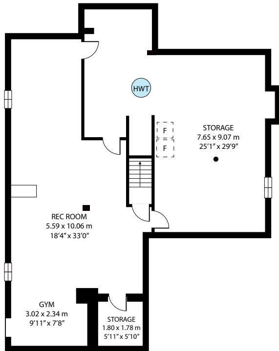
BASEMENT
